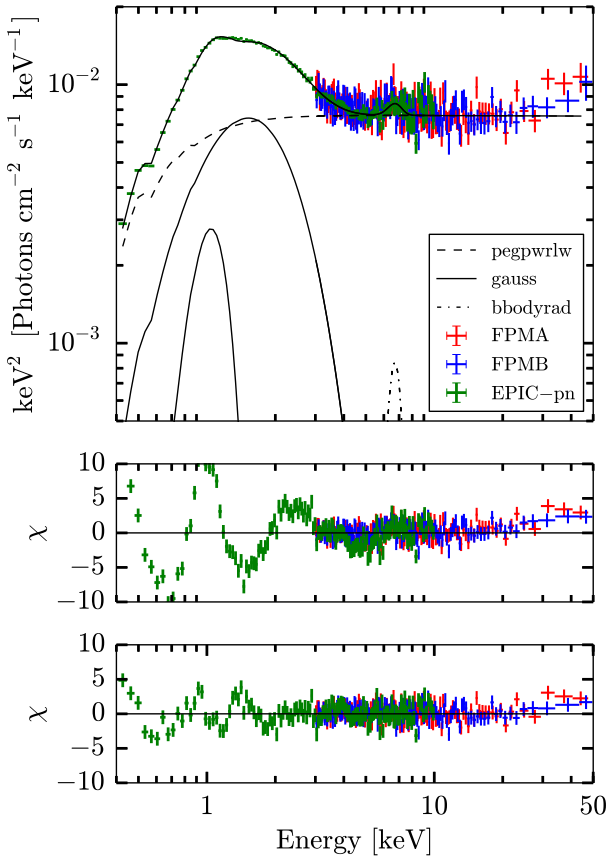
Figure 1. Top: The 2016 XMM-Newton EPIC-pn (green) and NuSTAR FPMA (red) and FPMB (blue) spectra unfolded around the best-fitting phenomenological model \text{CONSTANT}^*\text{TBABS}^*(\text{BBODYRAD}+\text{PEGPWRLW}+\text{GAUSS}+\text{GAUSS}) . The FPMB and EPIC-pn spectra have been rescaled by their fitted cross-calibration constant for visual clarity. Middle: \chi for the phenomenological model in D17, showing a broad Fe K \alpha feature and an emission feature around \sim 1 keV. Bottom: \chi for the best-fitting phenomenological model. We discuss the residuals remaining below 2 keV in detail in Section 4.
