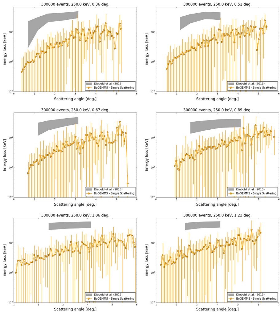
Fig. 15 The proton energy loss as a function of the scattering angle at E_0 = 250 keV in the 0.36^\circ - 1.23^\circ incident angle range
