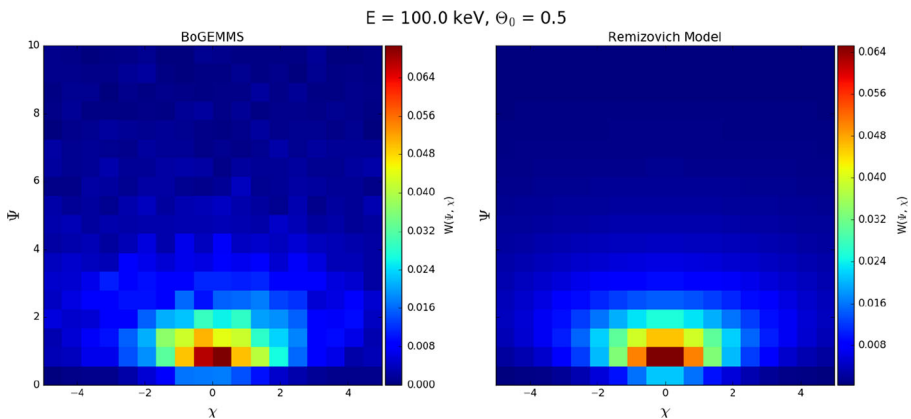
Fig. 3 Comparison between the bi-dimensional Remizovich angular distribution W(\Psi, \chi) of scattered protons obtained by the BoGEMMS simulation (left panel) and the analytical model (right panel) for an incident energy and polar angle of 100 keV and 0.5^\circ
