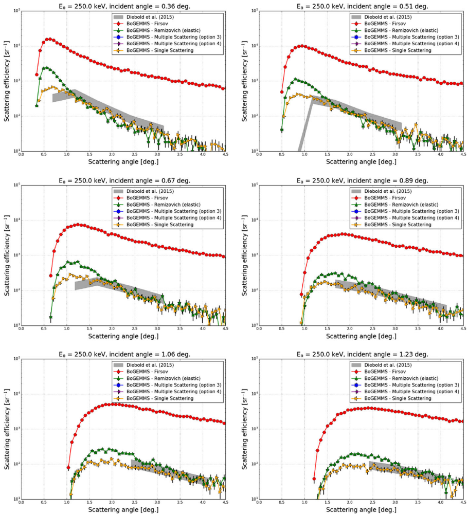
Fig. 12 Scattering efficiency at E_0 = 250 keV for an incident angle ranging from 0.36^\circ to 1.23^\circ
