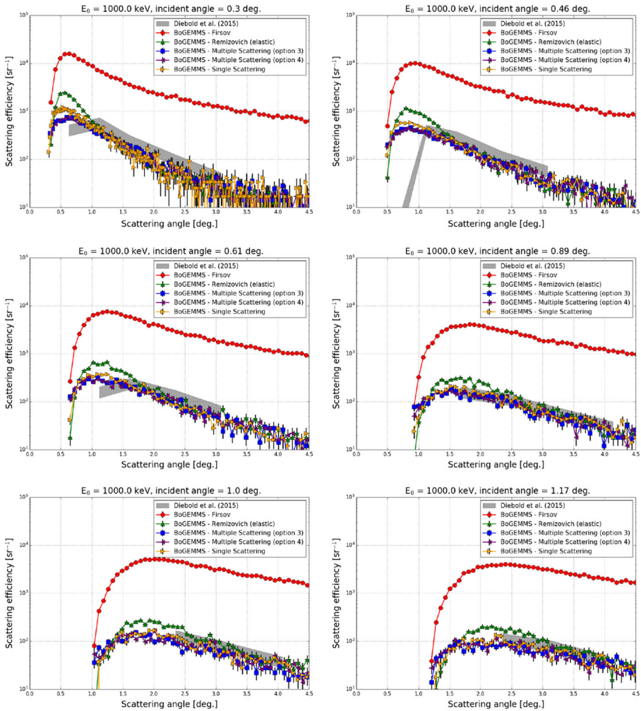
Fig. 14 Scattering efficiency at E_0 = 1000 keV for an incident angle ranging from 0.3^\circ to 1.17^\circ
