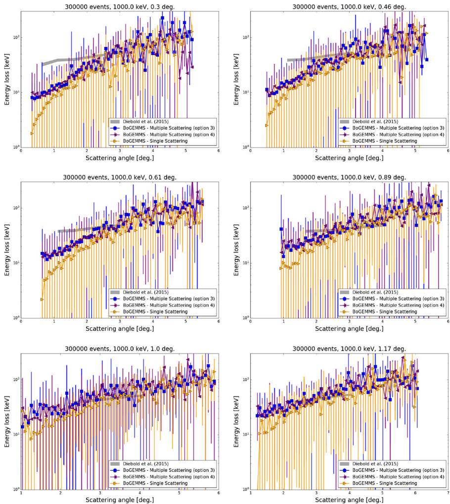
Fig. 17 The proton energy loss as a function of the scattering angle at E_0 = 1000 keV in the 0.3^\circ - 1.17^\circ incident angle range
