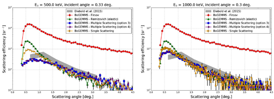
Fig. 8 Left panel: Scattering efficiency at E_0 = 500 keV for an incident angle of 0.33^\circ . Right panel: Scattering efficiency at E_0 = 1000 keV for an incident angle of 0.3^\circ
