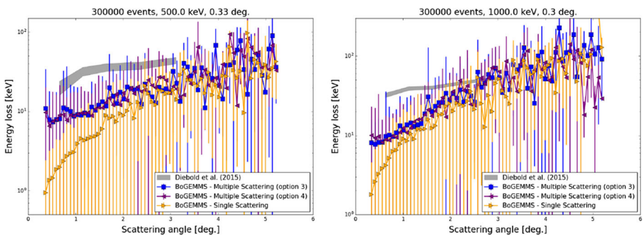
Fig. 11 Left panel: The proton energy loss as a function of the scattering angle at E_0 = 500 keV for an incident angle of 0.33^\circ Right panel: The proton energy loss as a function of the scattering angle at E_0 = 1000 keV for an incident angle of 0.3^\circ
