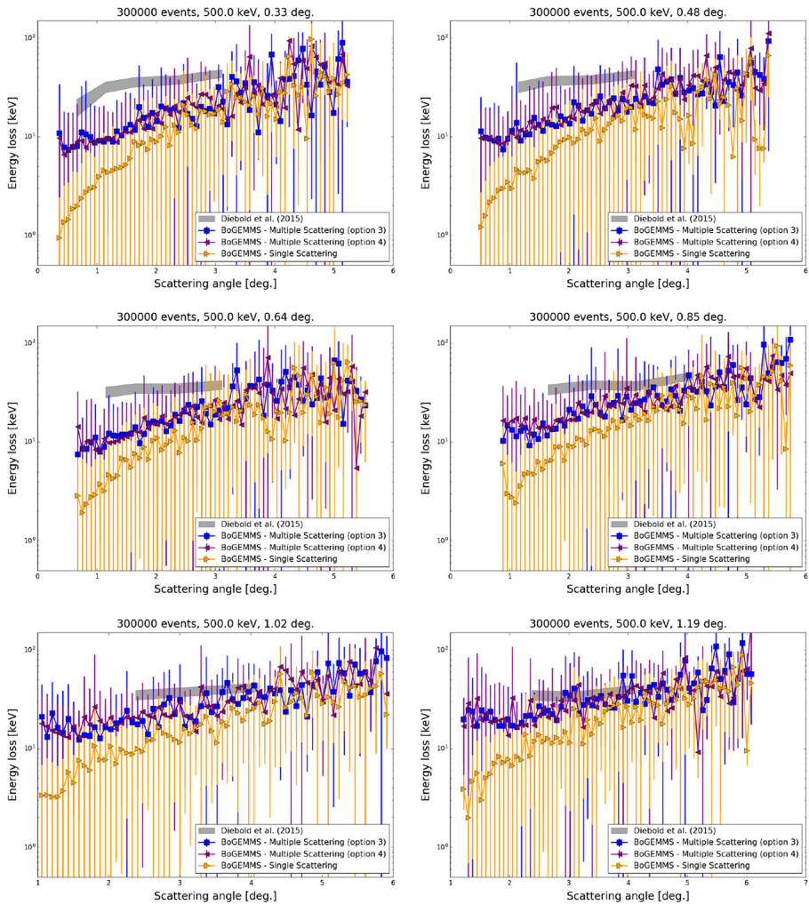
Fig. 16 The proton energy loss as a function of the scattering angle at E_0 = 500 keV in the 0.33^\circ - 1.19^\circ incident angle range
