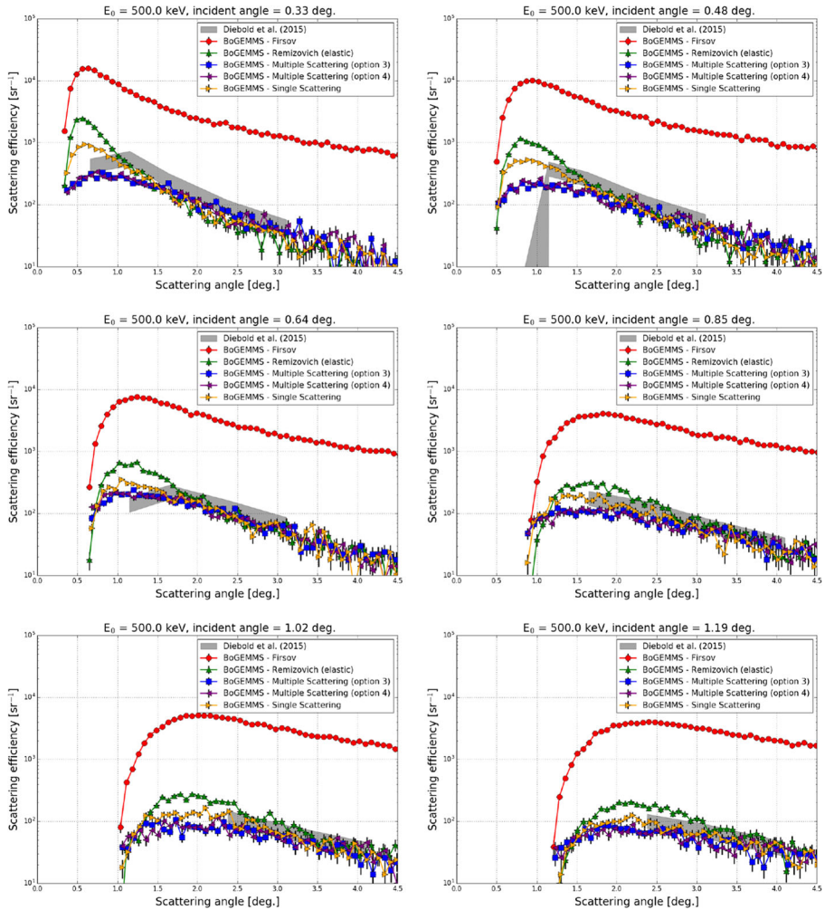
Fig. 13 Scattering efficiency at E_0 = 500 keV for an incident angle ranging from 0.33^\circ to 1.19^\circ
