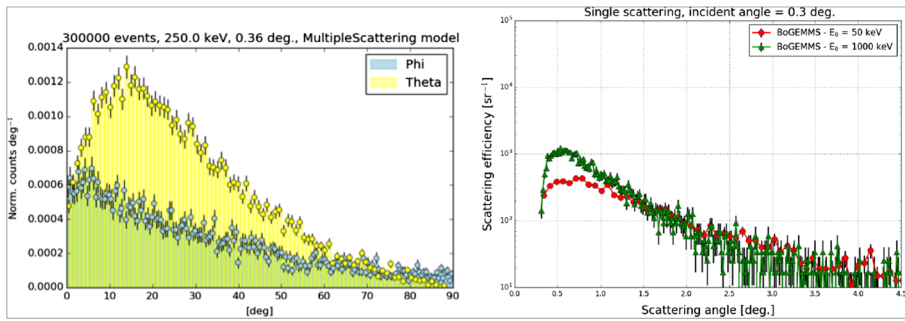
Fig. 9 Left panel: The angular distribution in \theta (yellow points) and \phi (light blue points) of scattered protons if multiple scattering is used as physics interaction. Right panel: Single scattering efficiency at E_0 = 50 and 1000 keV for an incident angle of 0.3^\circ
